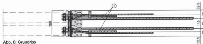
Abb. 6: Grundriss
