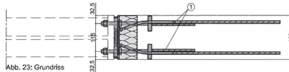
Abb. 23: Grundriss
